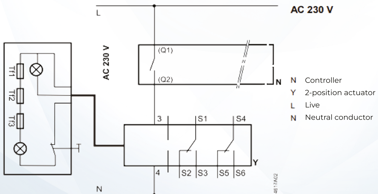
Wiring diagram for Siemens GRA326.1E/T12 actuator
