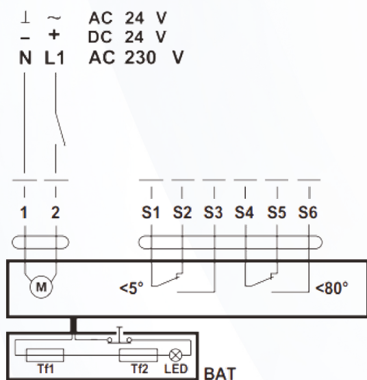
Wiring diagram for Belimo BFL 230-T, BFN 230-T actuators
