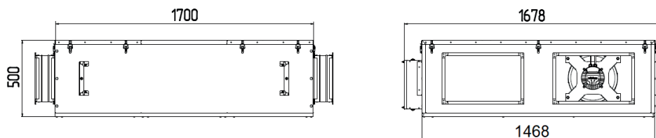
Fig. 9 SlimStar 1500 dimensions
