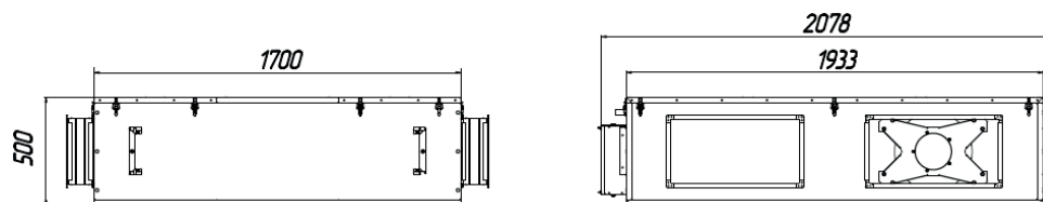
Fig. 10 SlimStar 2000 dimensions
