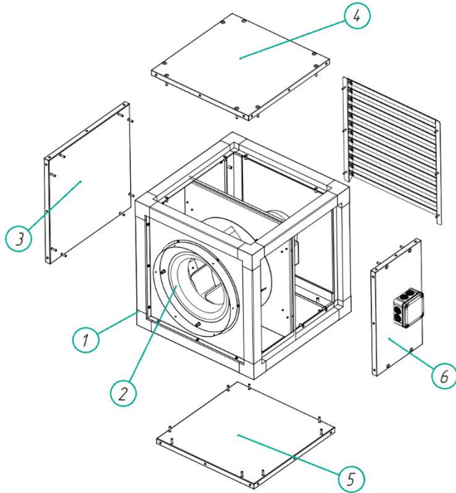
Picture 3 Design of the fan
