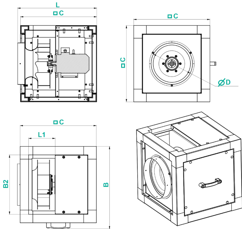
Picture 1 Dimensions KFS
