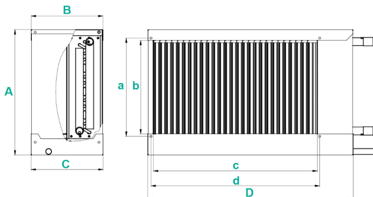
Figure 1 – Overall and Connection Dimensions
